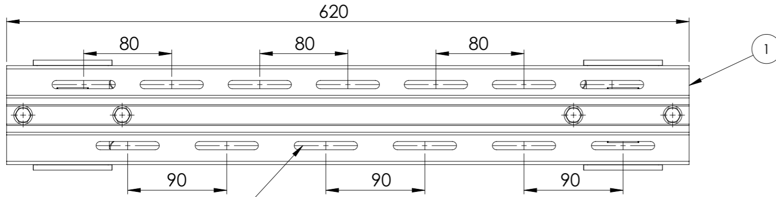
FRONT VIEW
