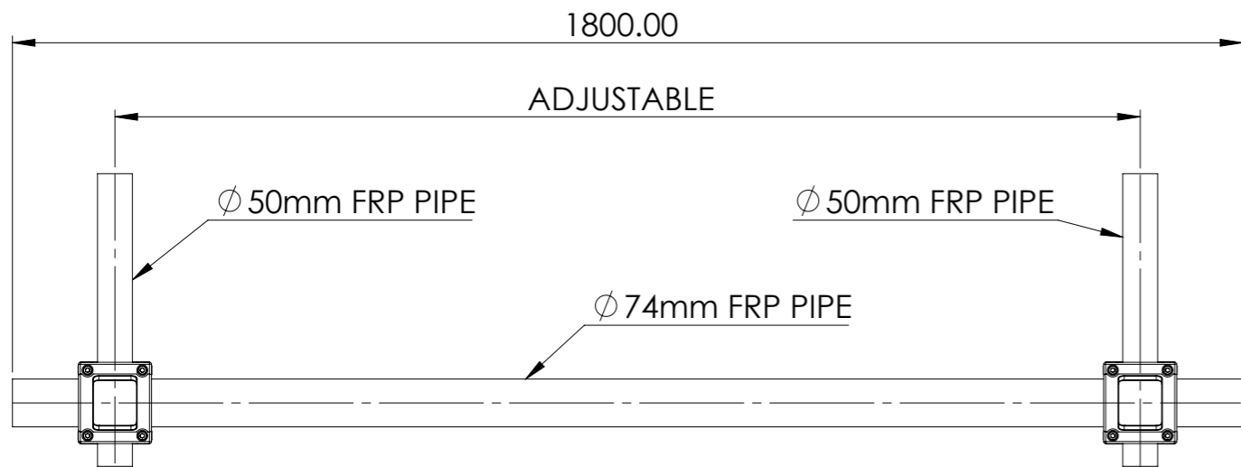
FRONT VIEW
